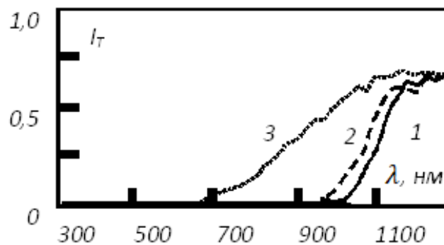
Figure-3. Graph of correlation of light transmittance of a silicon wafer of different thickness to the wavelength of light: 1 – d = 200 \mu\text{m} ; 2 – d = 100 \mu\text{m} ; 3 – d = 10 \mu\text{m} .
