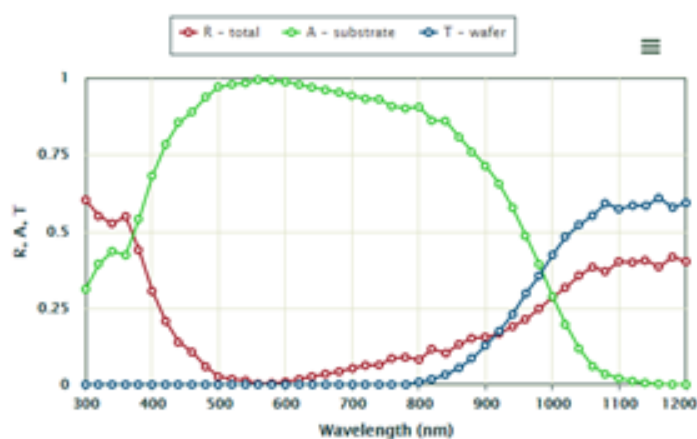
Figure-1. Spectral graph of light wavelength dependence of light reflection, absorption and conduction index for a crystalline silicon wafer with thickness d = 200\ \mu\text{m} .
