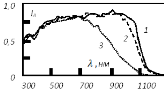
Figure-2. Graph of correlation of light absorption index of light absorption index of silicon wafers of different thicknesses: 1 – d = 200 \mu\text{m} ; 2 – d = 100 \mu\text{m} ; 3 – d = 10 \mu\text{m} .
