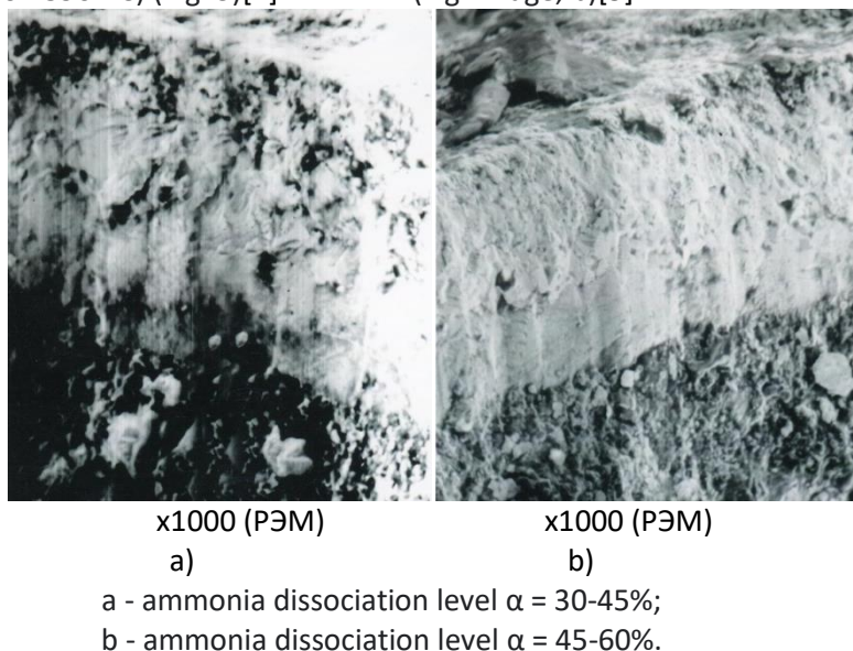
Figure 3 - Microstructure of Stal 45 after nitriding at 580°C for 3 hours.
